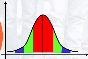
Bell's Graph
